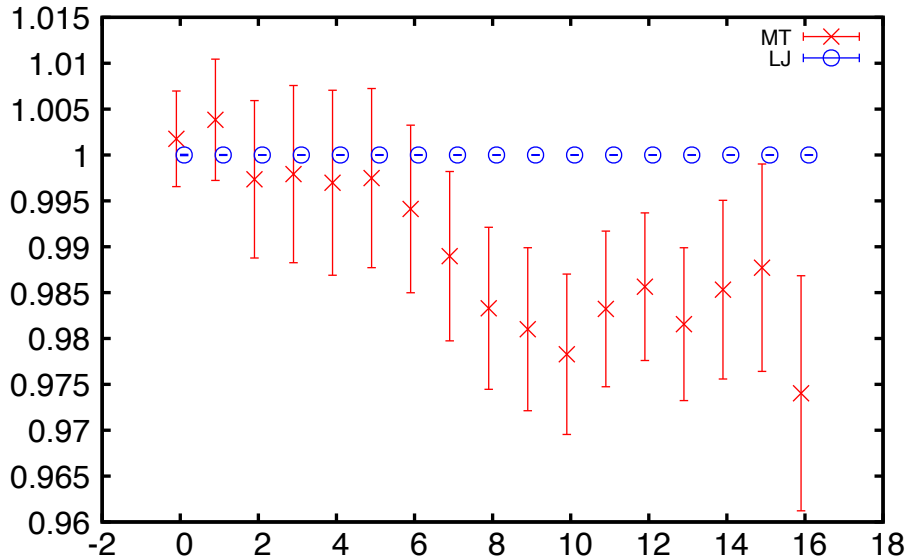
C(t) / C_{LJ}(t) , kaon000
