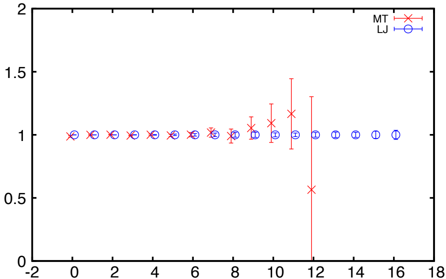
C(t) / C_{LJ}(t) , pion2pt001
