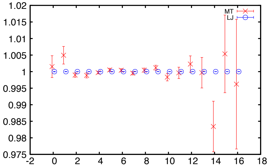
C(t) / C_{LJ}(t) , pion2pt000
