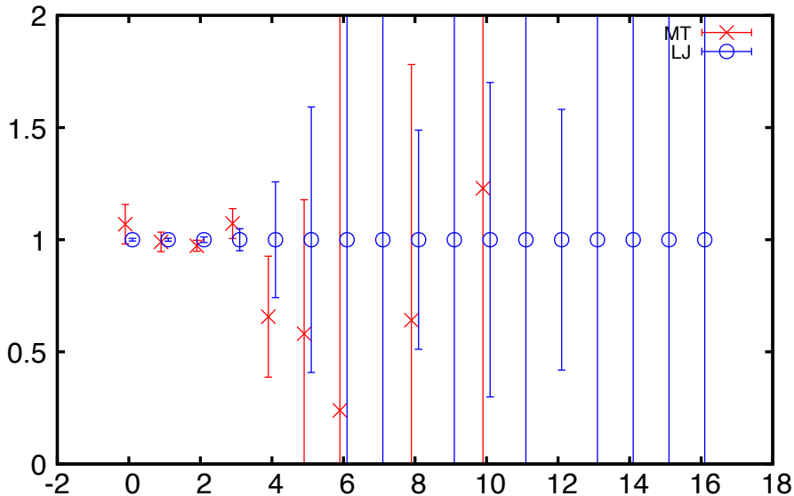
C(t) / C_{LJ}(t) , pion2pt111
