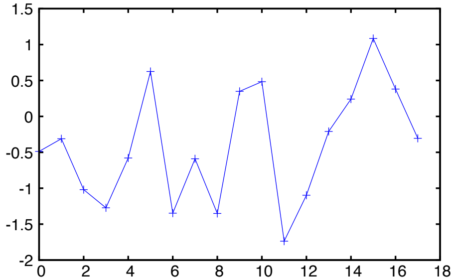
Deviation ( \sigma ), p ππ011 p ππ111
