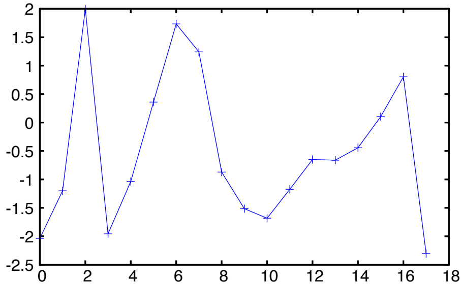
Deviation ( \sigma ), p 111 p 000
