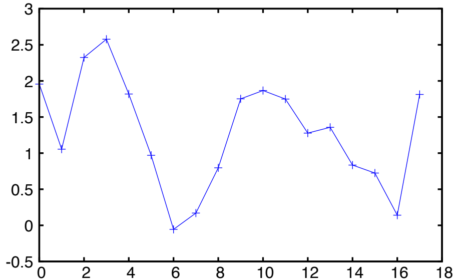
Deviation ( \sigma ), p ipi111 KK typeV
