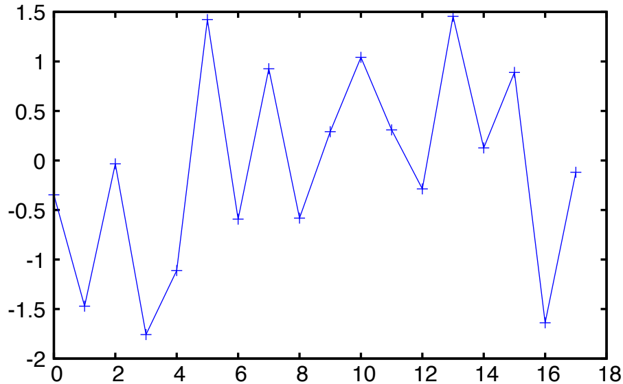
Deviation ( \sigma ), p ππ011 p ππ011
