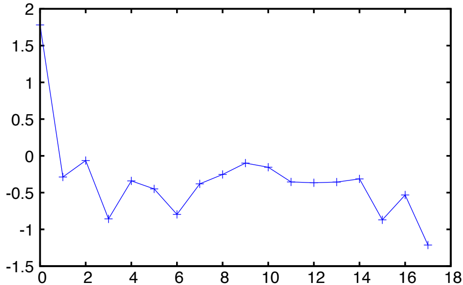
Deviation ( \sigma ), ppi001 ppi000
