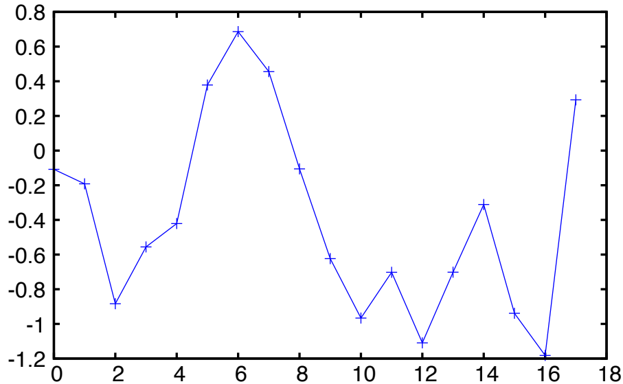
Deviation ( \sigma ), ppi000 ppi000
