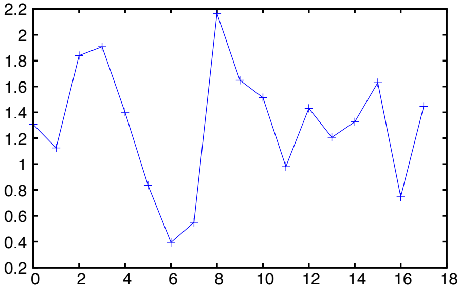
Deviation ( \sigma ), pipi111 pipi001 typeV
