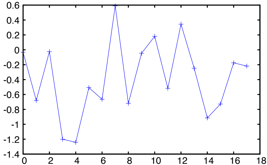
Deviation ( \sigma ), ppi001 ppi011 typeR
