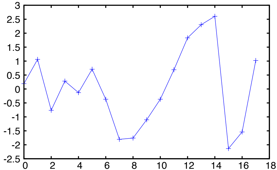
Deviation ( \sigma ), pipi000 pipi011
