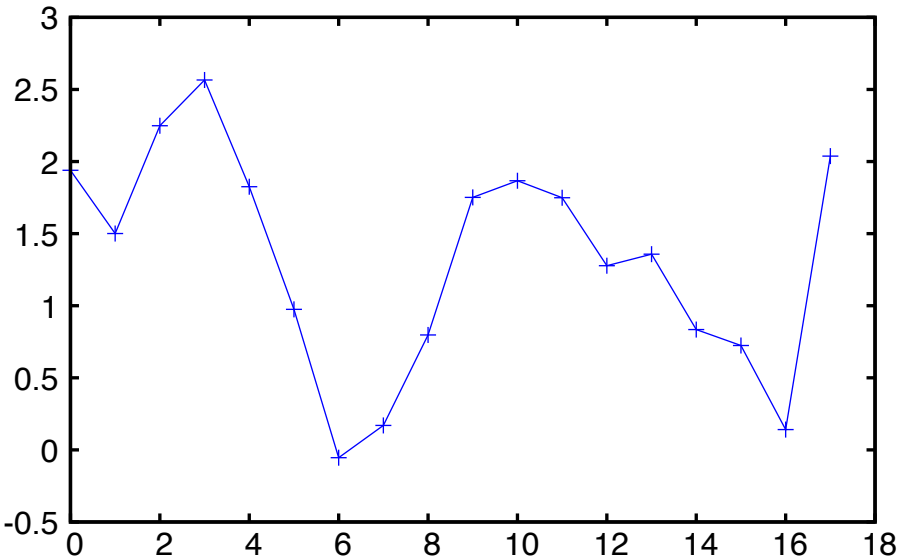
Deviation ( \sigma ), pipi111 KK vacUnsubt
