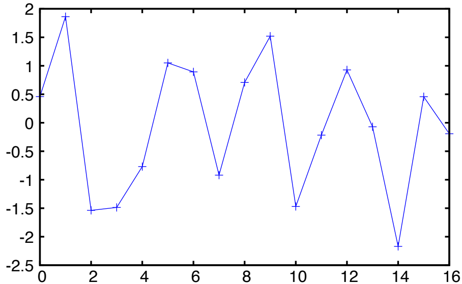
Deviation ( \sigma ), pion2pt000
