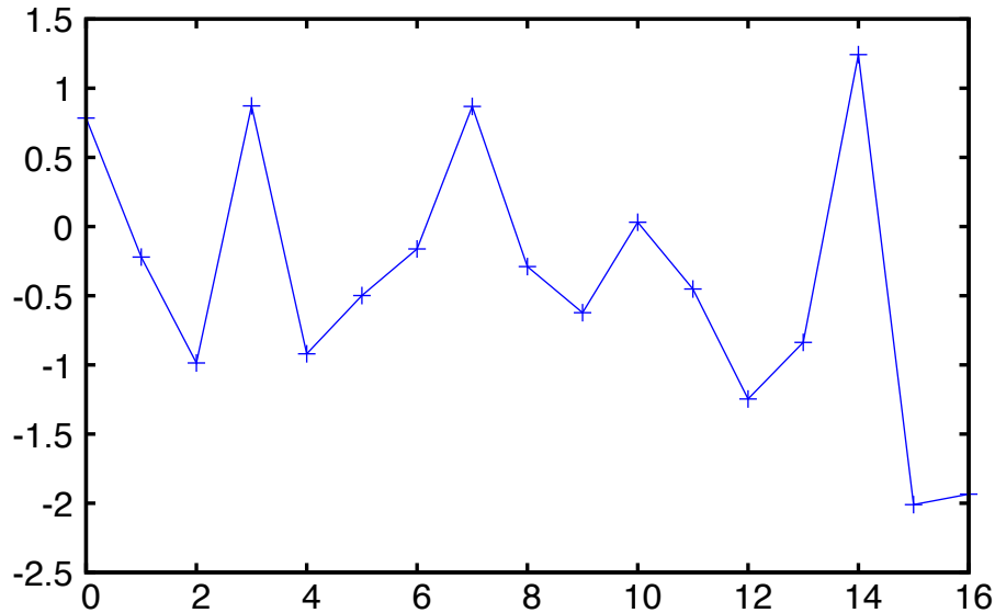
Deviation ( \sigma ), pion2pt111
