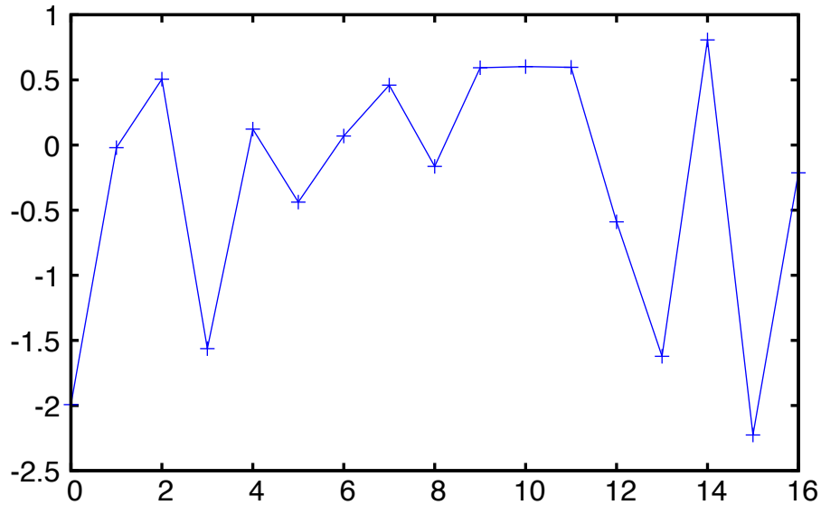
Deviation ( \sigma ), pion2pt001
