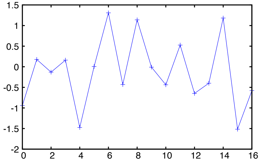
Deviation ( \sigma ), pion2pt011
