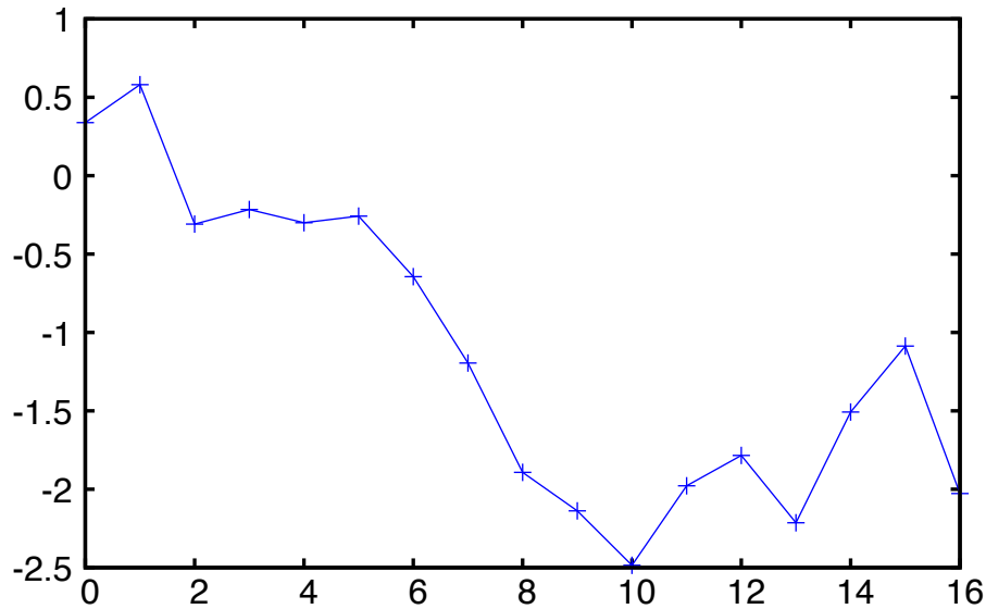
Deviation ( \sigma ), kaon000
