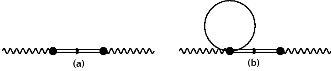
Figure 3: The diagrams that contribute to the photon vacuum polarization with the \rho in S\chi PT at (a) tree level and (b) one loop. The double line is the vector mesons and the single line is a pion or kaon as before.
