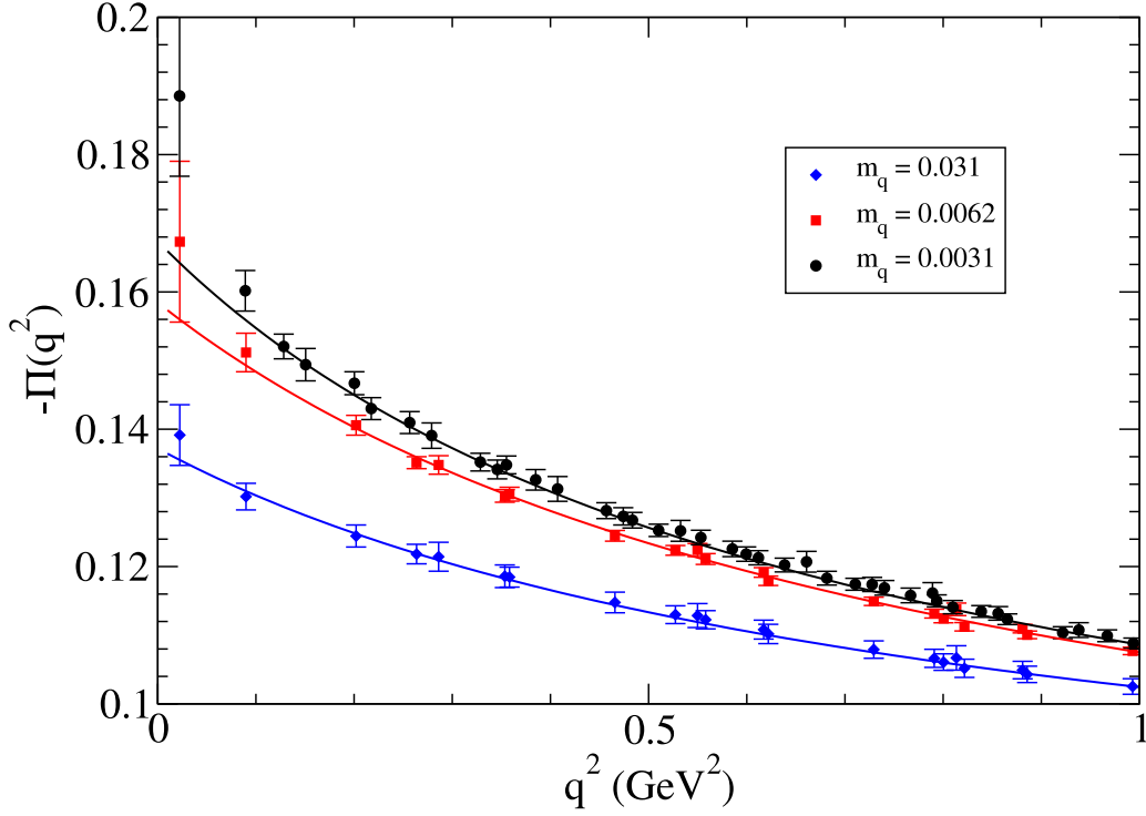
Figure 4: Fits to the lattice data using the tree-level vector formula for the three different quark masses for the low- q^2 region.
