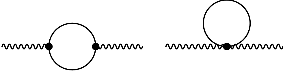
Figure 2: The two diagrams that contribute to the photon vacuum polarization at one loop in S\chi PT.
