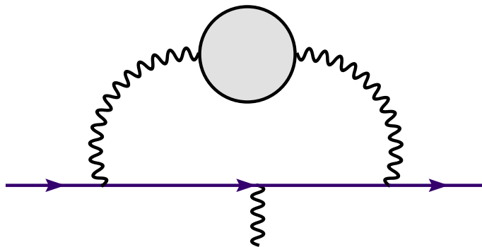
Figure 1: The lowest order hadronic contribution to the muon g-2 . The blob represents all QCD diagrams.
