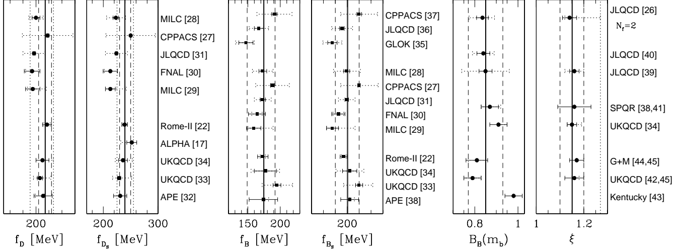
Fig. 2. Recent results for decay constants and B -parameters in the quenched approximation, compared to the global averages of eqs.(11), (12), (15), (17) and (18) (solid vertical lines). For D -mesons the dashed lines indicate the statistical error, while the systematic error is represented by the dotted lines. For the B -system the dashed vertical lines denote the total error, with the uncertainty due to chiral logs included in quadrature. Dotted error bars on individual determinations indicate the quoted systematic error. The result for B_B and \xi in [26] was obtained for N_f = 2 .
