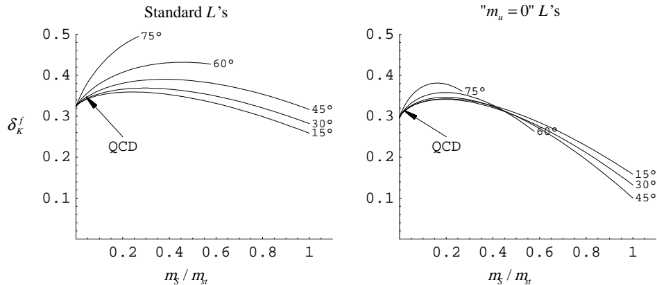
Fig. 2. \delta_K^f along rays of fixed angle in the contour plots.
