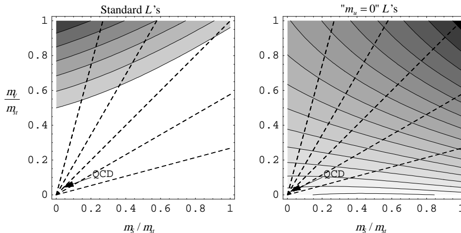
Fig. 1. Contour plots of \delta_K^M . The x- and y-axes are the light sea and valence quark masses, respectively, in units of the physical strange quark mass. In the left-hand plot, the white region has 0 < \delta_K^M < 0.1 , and the contours increase from 0.1 to 0.2 (upper left) in steps of 0.02. In the right-hand plot the contours start at 0.475 (lower left) and increase to 0.825 in steps of 0.025.
